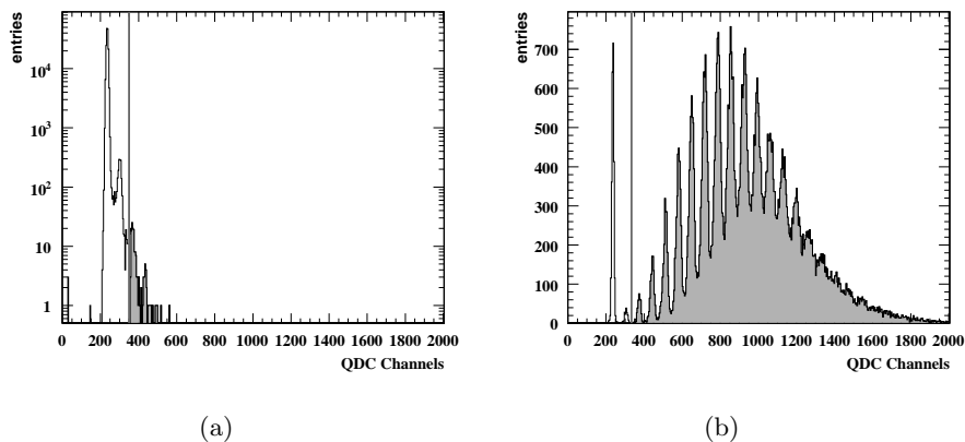
Fig. 2. – Scintillator crystal read out by a 400 pixels MPPC. A threshold (the vertical line in the figure) is defined from the pedestal, so that the noise above it is 3 kHz (grey area in (a)). This threshold in amplitude defines the efficiency of the collection of the signal (b): in gray is the part of the signal above the cut, which is 98% of the total, after subtracting the pedestal contribute.
