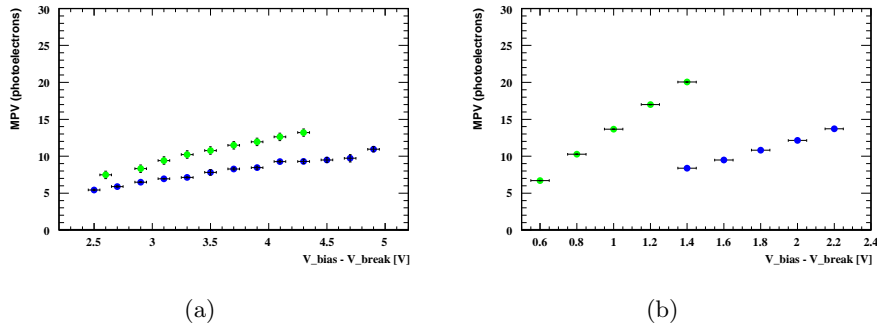
Fig. 3. – Most probable value of a mip spectrum detected by a 1600 pixels (a) and a 400 pixels (b) MPPC. The blue dots correspond to the direct coupling, while the green ones to the wavelength shifting mediated readout.
