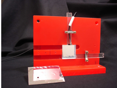
Fig. 1. – Setup for the direct coupling. The scintillator is installed in a specific housing. The MPPC is fixed at one end of a plastic holder which can be located in two different positions. The coupling is reproducible at a 3% level.
