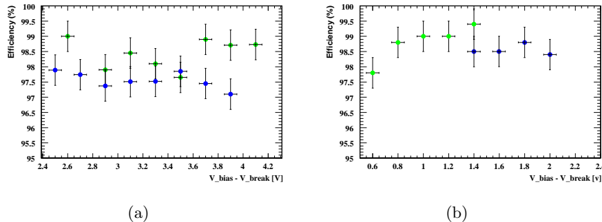
Fig. 4. – Signal collection efficiency for the 1600 pixels (a) and 400 pixels (b) MPPCs. The blue points correspond to the direct coupling, while the green points refer to the wavelength shifting mediated readout.
